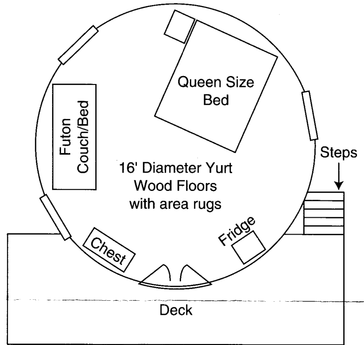
Sample Yurt Layout
